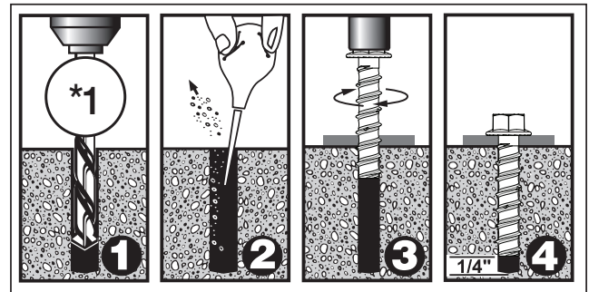
*1 : Anchor nominal diameter equals drill bit size
